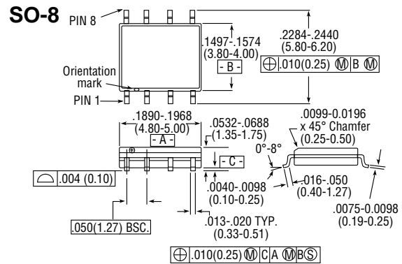
8-Lead SOP outline dimensions Narrow body .150
