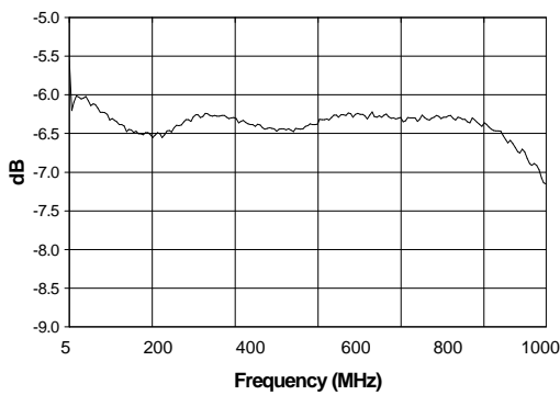
Conversion Loss
