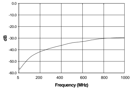
L-R Isolation
