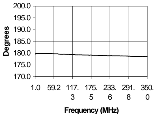
Phase Unbalance
