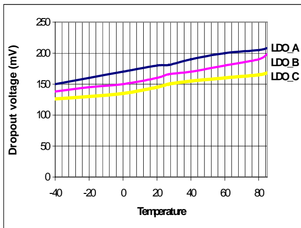
Figure 9. Dropout voltage temperature dependency with maximum output current.
