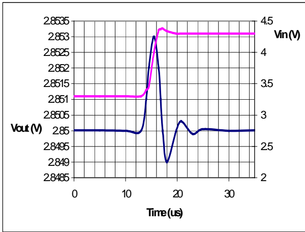
Figure 2. LDO_C line transient for 1 V change at supply voltage.
