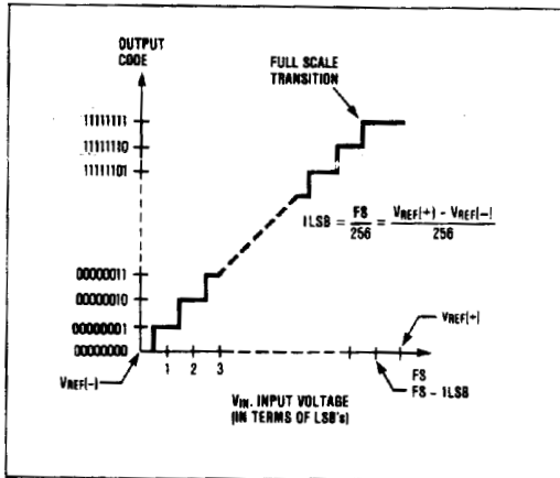
Figure 6. Transfer Function
