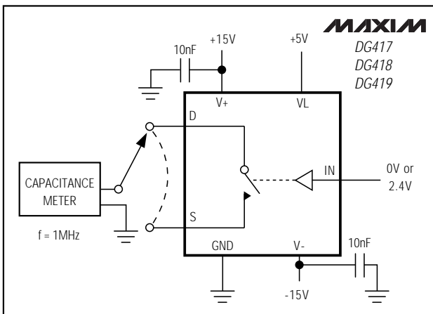
Figure 8. Drain-Source Off-Capacitance
