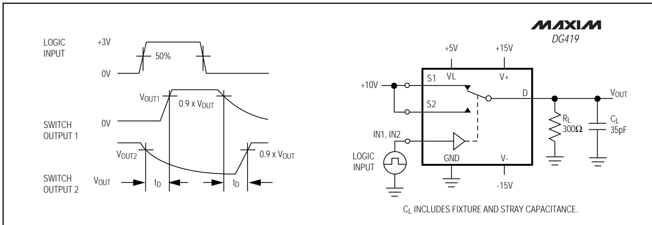
Figure 4. DG419 Break-Before-Make Interval
