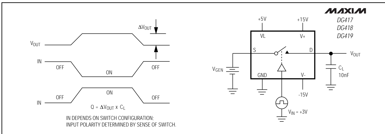
Figure 5. Charge Injection
