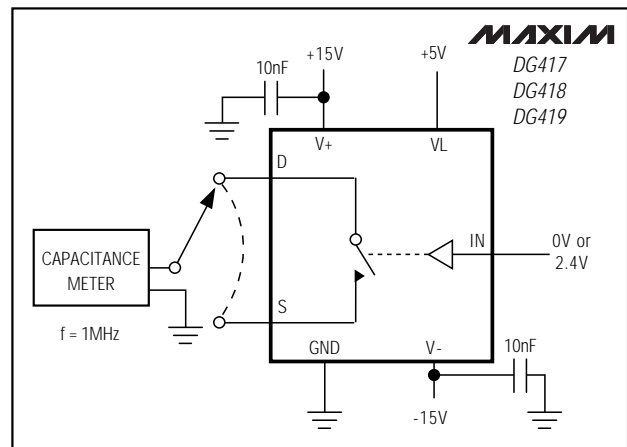
Figure 9. Drain-Source On-Capacitance
