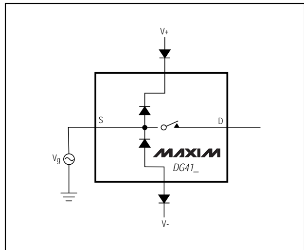
Figure 1. Overvoltage Protection Using External Blocking Diodes
