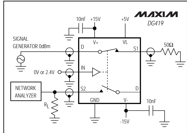
Figure 7. DG419 Crosstalk
