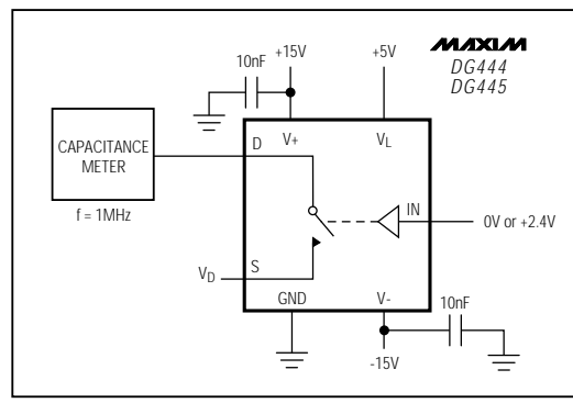
Figure 7. Source/Drain-On Capacitance
