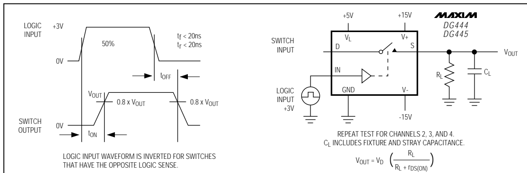
Figure 2. Switching Time
