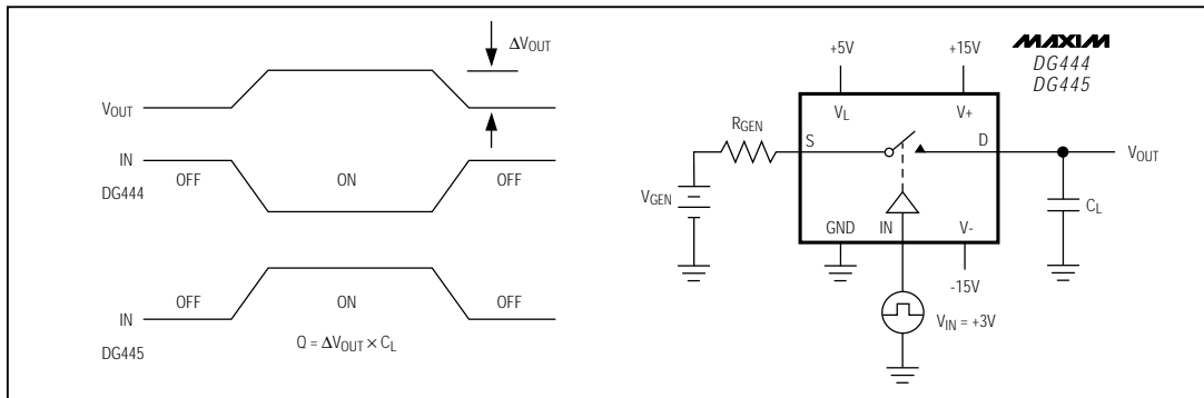
Figure 3. Charge Injection
