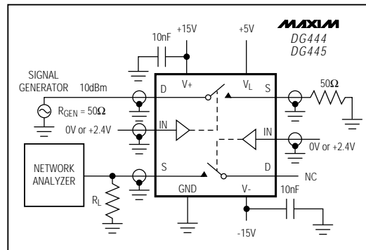
Figure 5. Crosstalk
