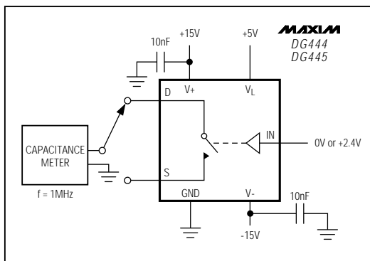
Figure 6. Source/Drain-Off Capacitance
