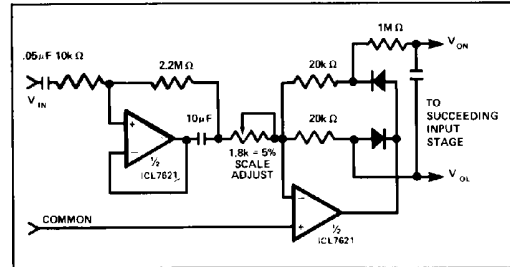
Figure 6. Averaging AC to DC Converter — Recommended for Maxim's ICL7106/107/109 A/D Converters.
