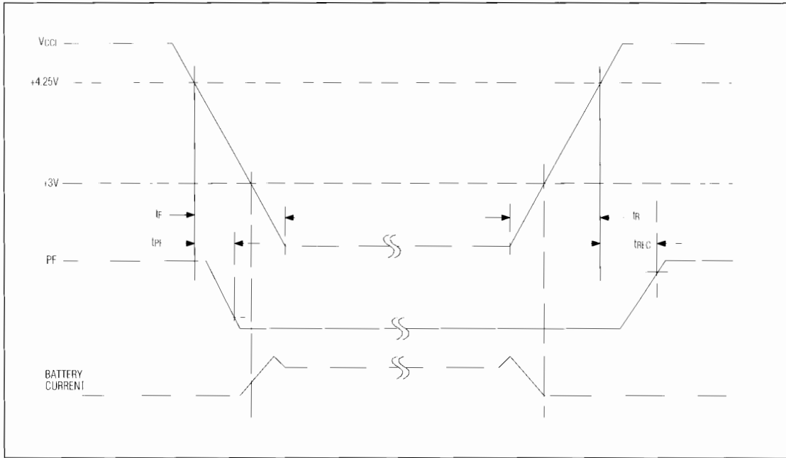
Figure 1. Power-Down/Power-Up Conditions
