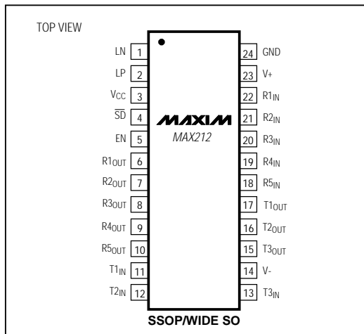
Pin Configuration
