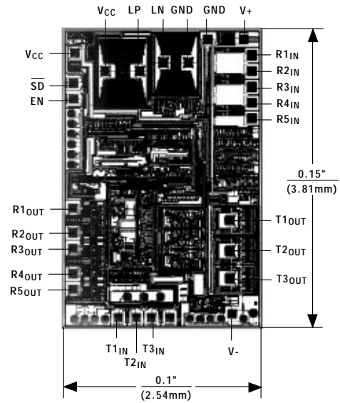
Chip Topography
