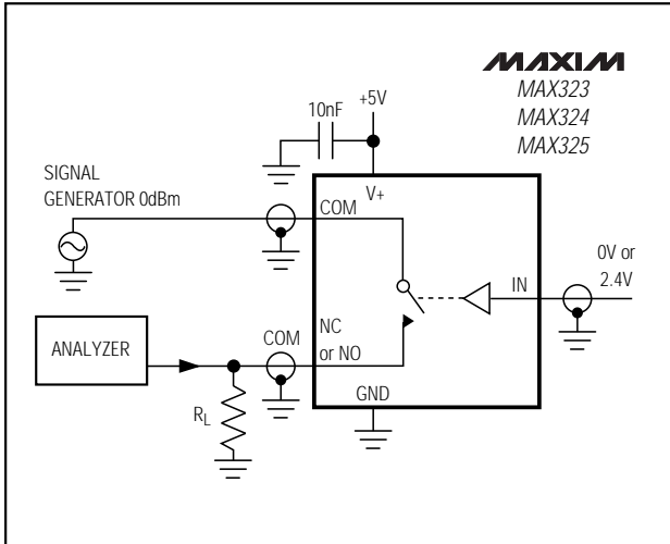
Figure 5. Off Isolation
