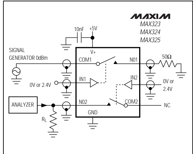
Figure 6. Crosstalk
