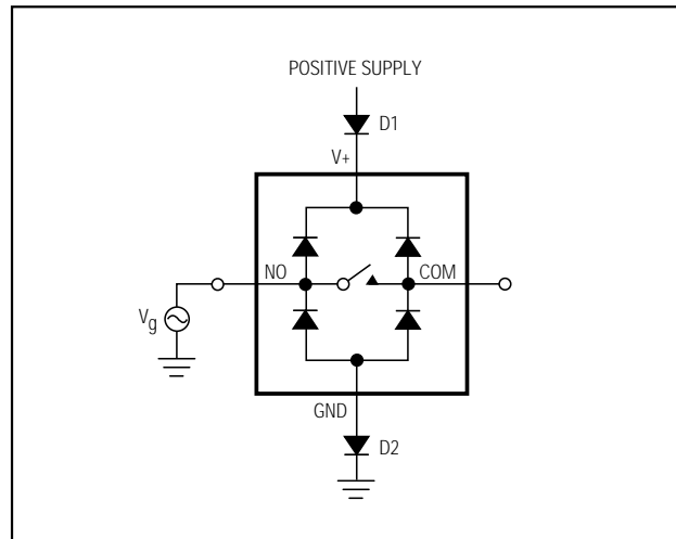
Figure 1. Overvoltage Protection Using Two External Blocking Diodes
