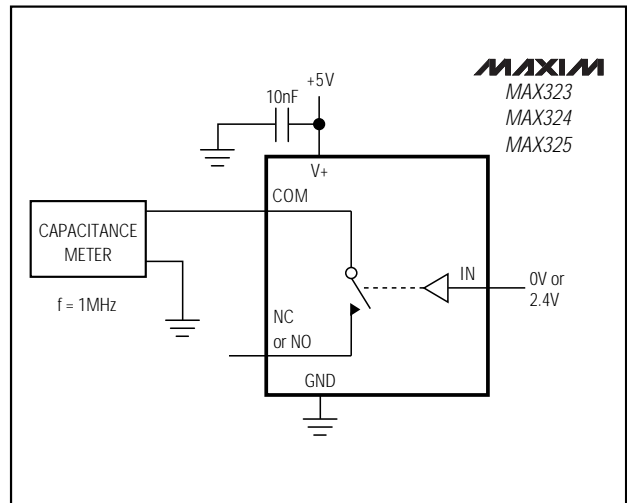
Figure 8. Channel-On Capacitance
