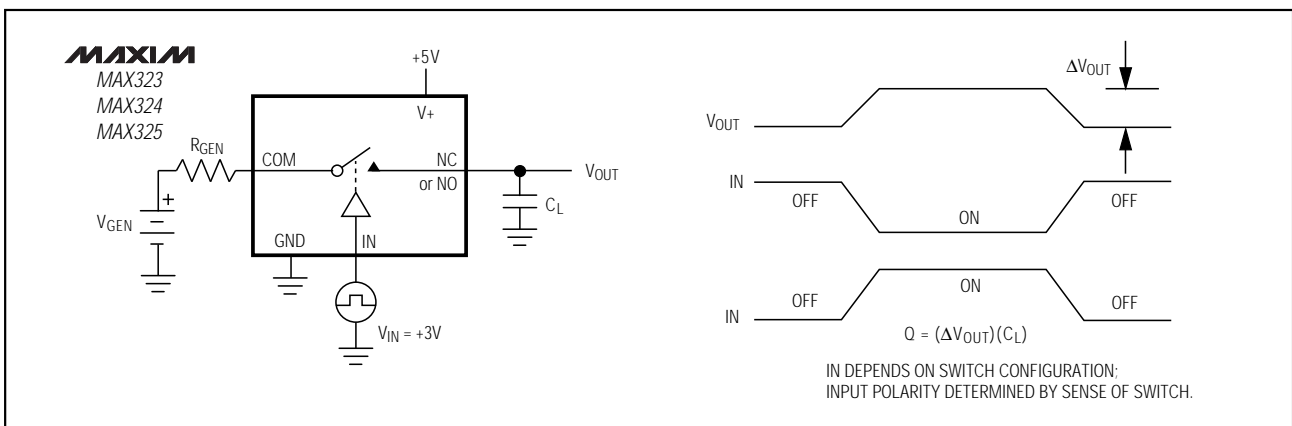
Figure 4. Charge Injection
