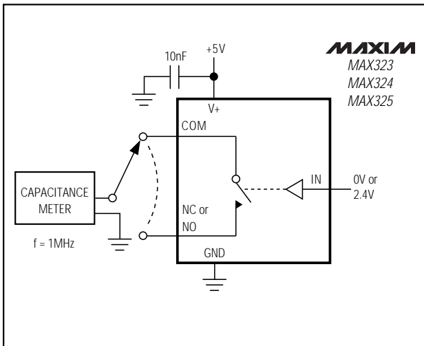
Figure 7. Channel-Off Capacitance
