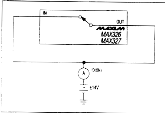
Figure 4. On Leakage Current Test Circuit
