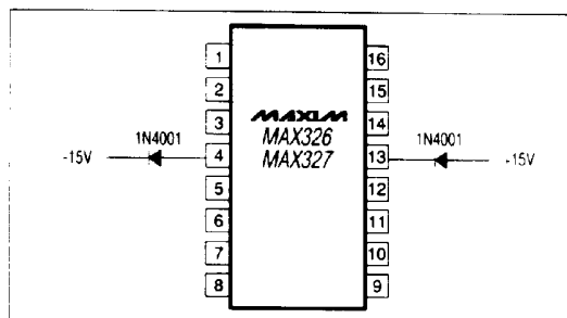
Figure 2. Protection Against Fault Conditions
