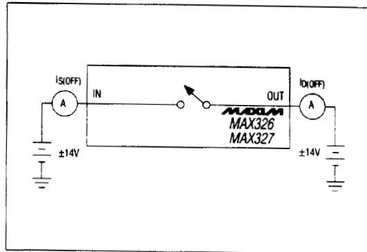
Figure 5. Off Leakage Current Test Circuit
