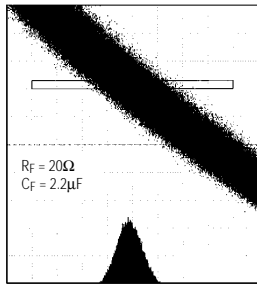
RECOVERED CLOCK JITTER (155Mbps, 2 7 -1 PRBS, 5.1ps RMS)
