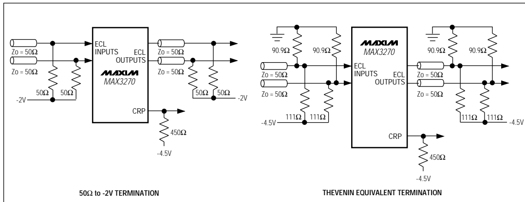
Figure 4. Typical Input and Output Terminations
