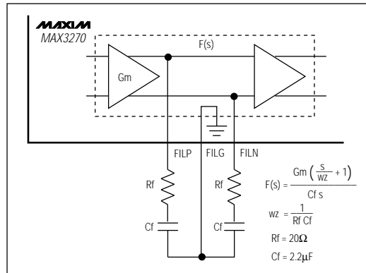
Figure 2. Loop Filter
