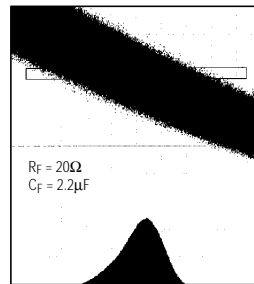
RECOVERED CLOCK JITTER (622Mbps 2 7 -1 PRBS 9.0ps RMS)
