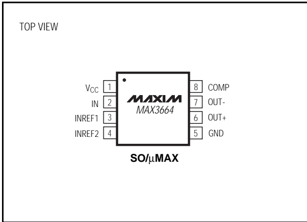
Pin Configuration
