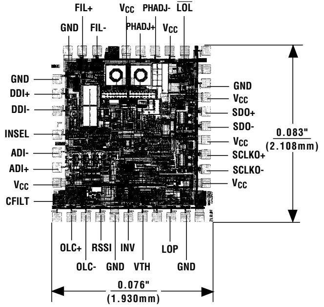
Chip Topography
