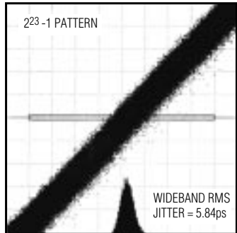
RECOVERED CLOCK JITTER
