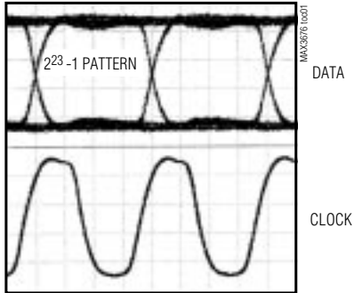
RECOVERED DATA AND CLOCK (SINGLE ENDED)
