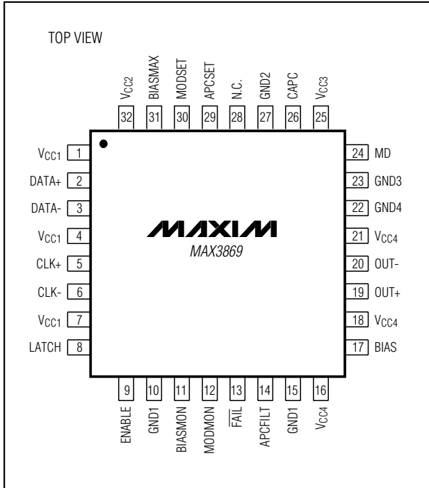
Pin Configuration
