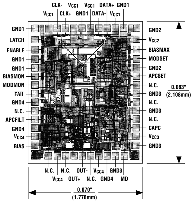
Chip Topography
