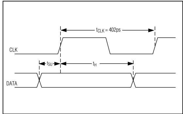
Figure 3. Setup/Hold Time Definition
