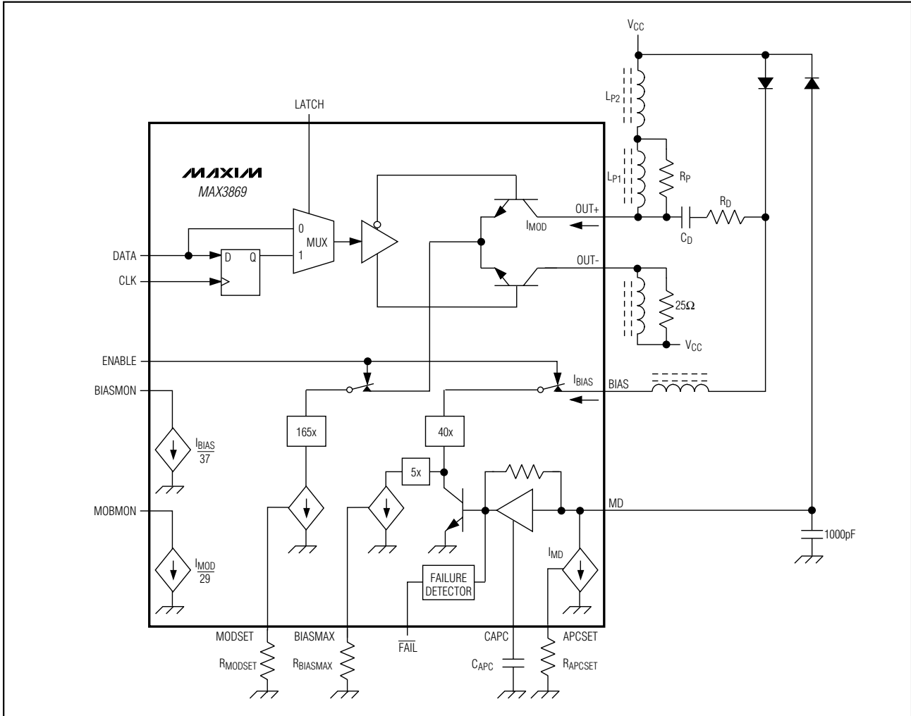
Figure 4. Functional Diagram
