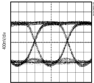
ELECTRICAL EYE DIAGRAM (I MOD = 60mA, 2 13 -1 +80 CID, 32 TQFP-EP)
