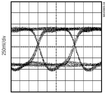
ELECTRICAL EYE DIAGRAM (I MOD = 30mA, 2 13 -1 +80 CID, 32 TQFP-EP)
