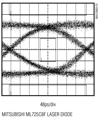
EYE DIAGRAM (2.488Gbps, 1300nm FP LASER, 1.87GHz FILTER, 32 TQFP-EP)
