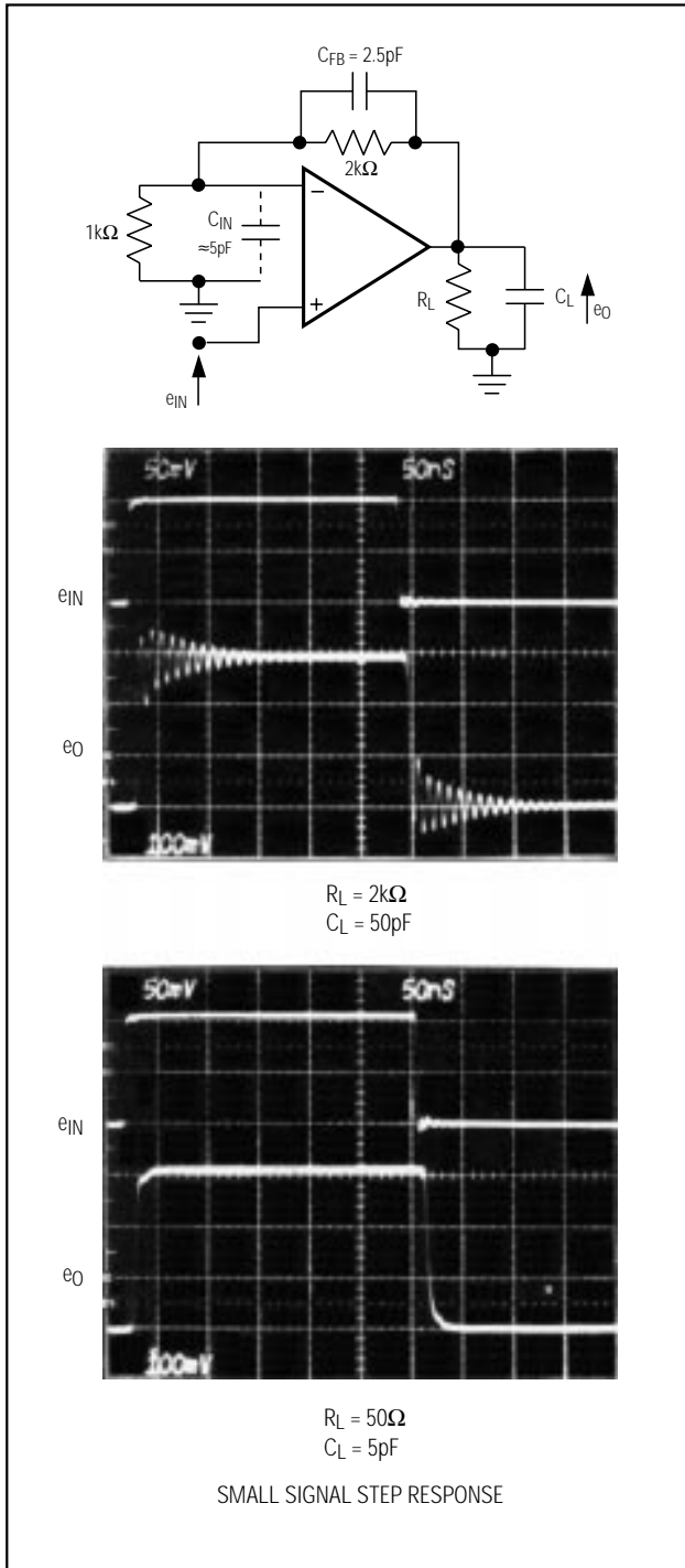
Figure 4. Response Characteristics with Input Pole Cancellation, A_V = 3
