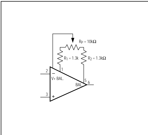
Figure 2. V_{OS} Nulling Method for MAX408
