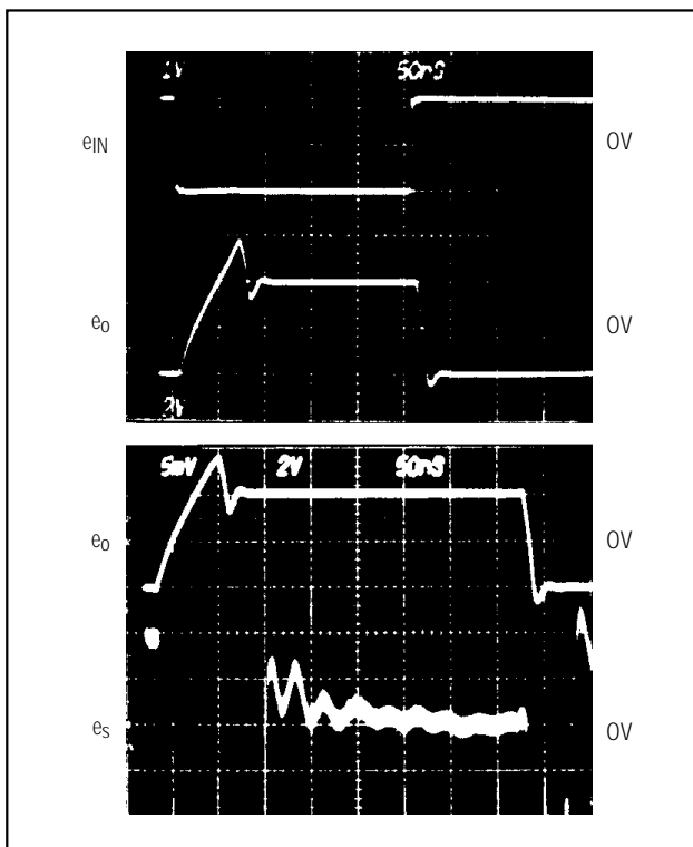
Figure 1B. Large Signal Response
