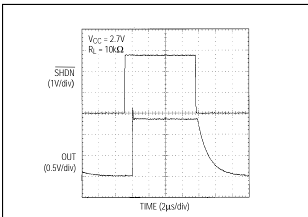
Figure 13. Shutdown Output Voltage
