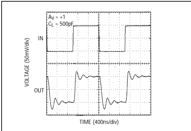
Figure 5. MAX4122/23/26/27/29 Small-Signal Transient Response with Capacitive Load
