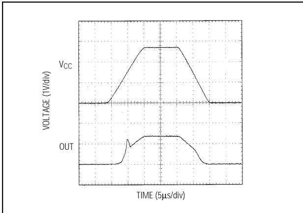
Figure 11. Power-Up Output Voltage
