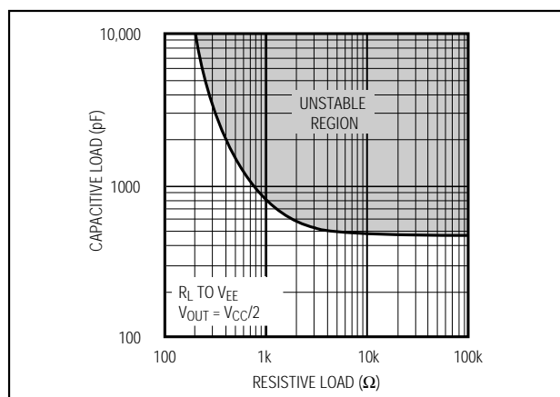
Figure 4. Capacitive-Load Stability
