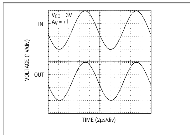
Figure 3. Rail-to-Rail Input/Output Voltage Range
