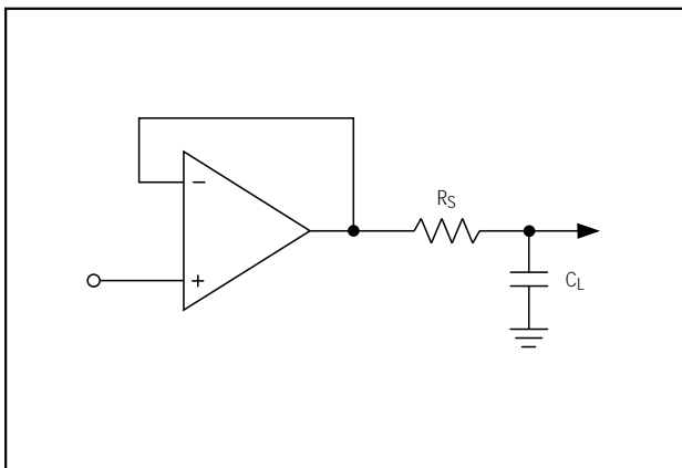
Figure 9. Capacitive-Load-Driving Circuit
