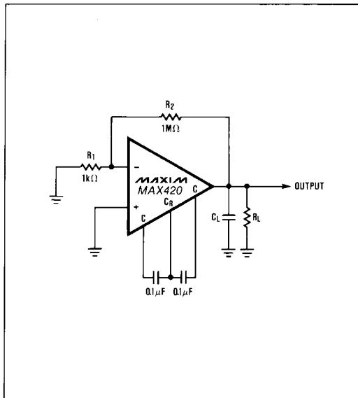
Figure 1. Test Circuit.
