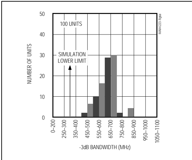
Figure 6a. MAX4224 -3dB Bandwidth Distribution
