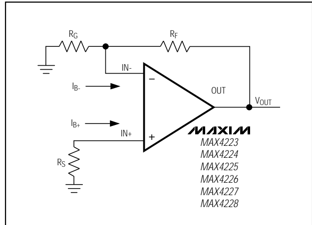
Figure 2. Output Offset Voltage
