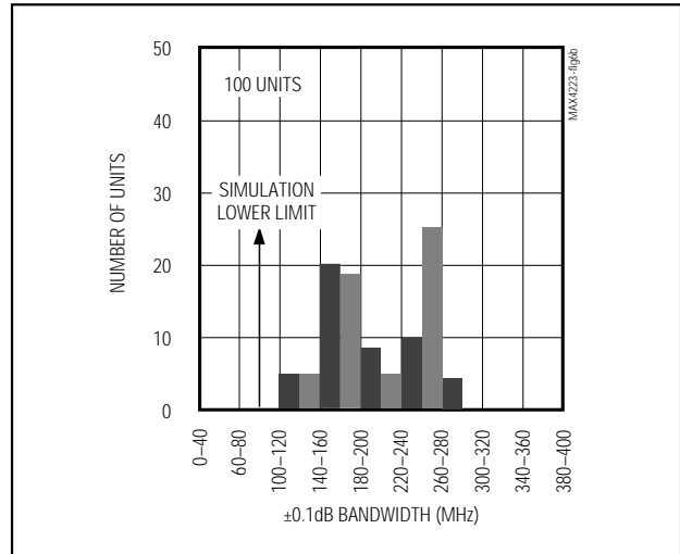
Figure 6b. MAX4224 ±0.1dB Bandwidth Distribution
