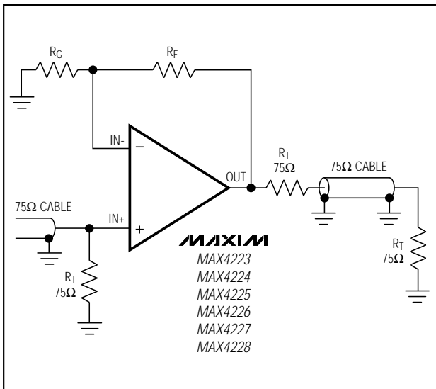
Figure 3. Video Line Driver
