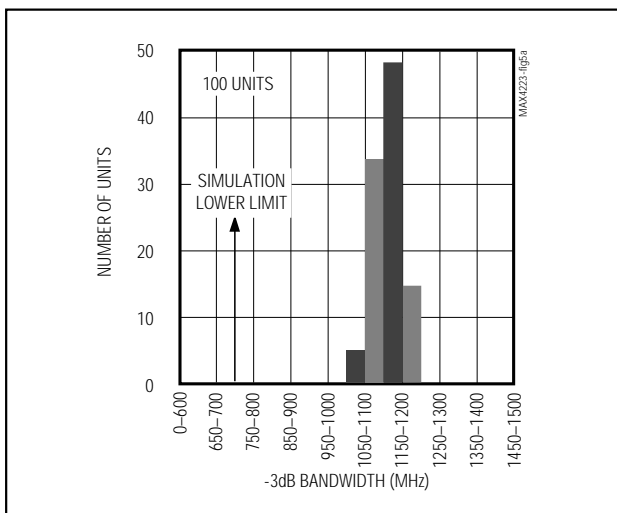
Figure 5a. MAX4223 -3dB Bandwidth Distribution
