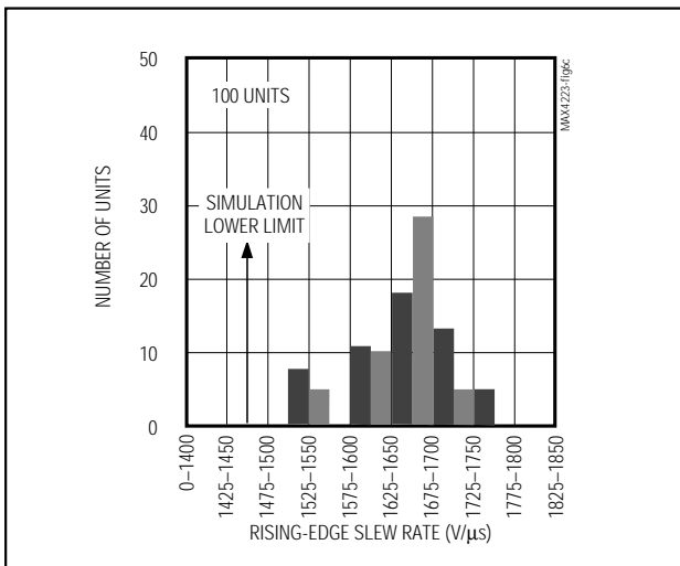
Figure 6c. MAX4224 Rising-Edge Slew-Rate Distribution
