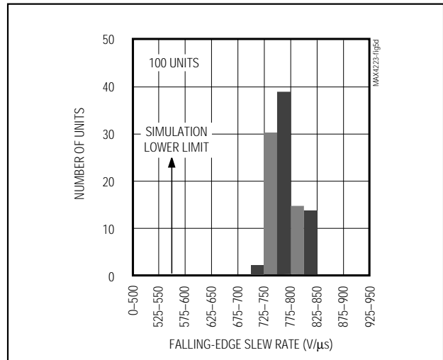
Figure 5d. MAX4223 Falling-Edge Slew-Rate Distribution
