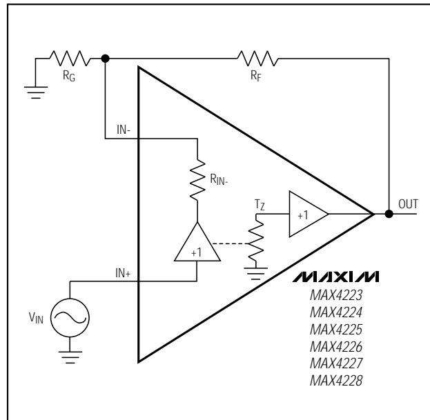
Figure 1. Current-Feedback Amplifier
