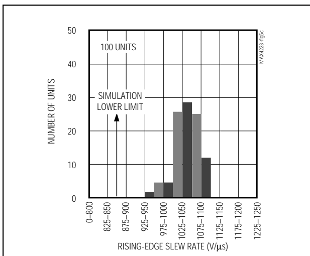
Figure 5c. MAX4223 Rising-Edge Slew-Rate Distribution
