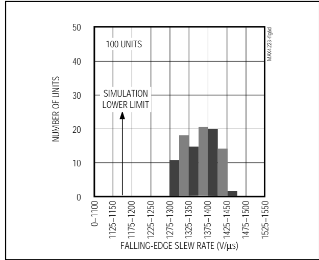
Figure 6d. MAX4224 Falling-Edge Slew-Rate Distribution
