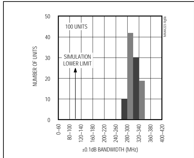
Figure 5b. MAX4223 ±0.1dB Bandwidth Distribution
