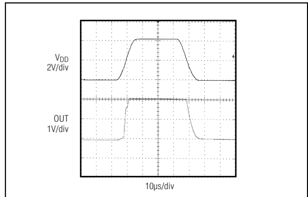
Figure 5. Power-Up/Power-Down Waveform
