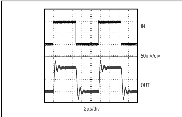
Figure 2. Small-Signal Transient Response with Excessive Capacitive Load
