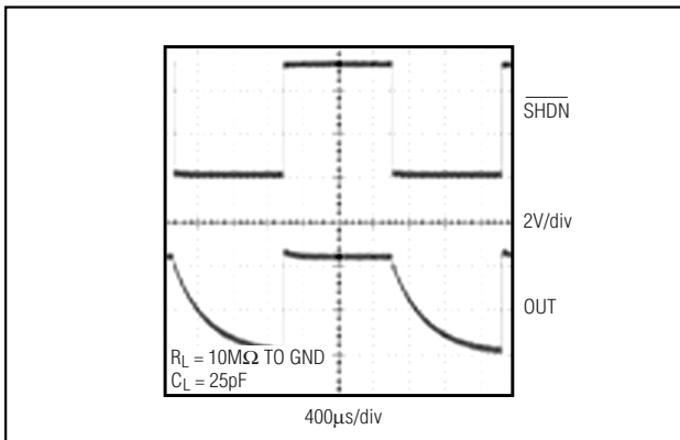
Figure 4. Shutdown Waveform
