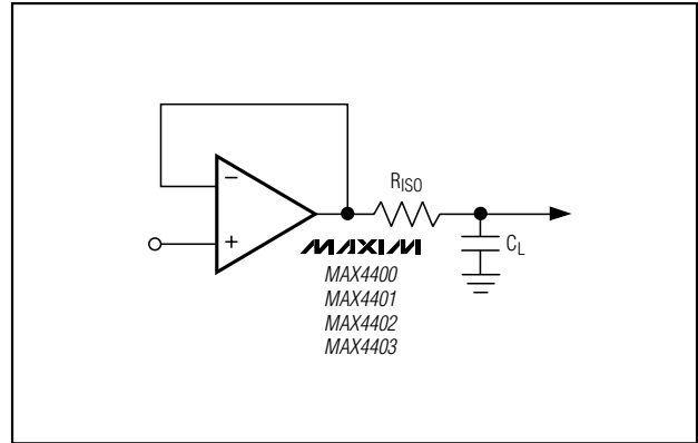
Figure 3. Capacitive-Load-Driving Circuit
