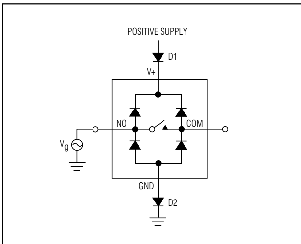
Figure 1. Overvoltage Protection Using Two External Blocking Diodes
