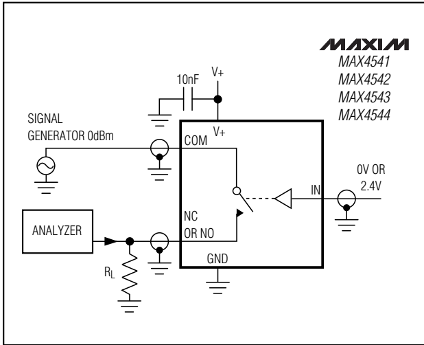
Figure 5. Off-Isolation
