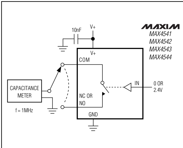
Figure 7. Channel Off/On-Capacitance
