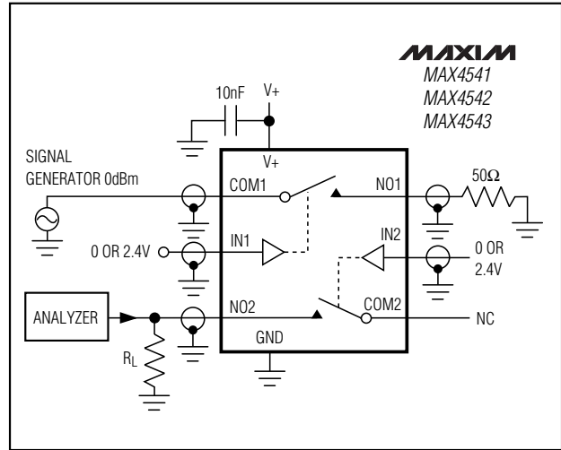
Figure 6. Crosstalk
