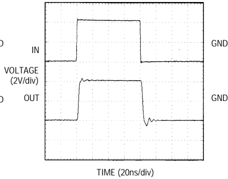
LARGE-SIGNAL PULSE RESPONSE ( A_{VCL} = +1V/V , C_L = 50pF )
