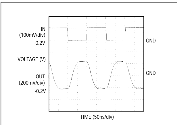
Figure 10a. 5MHz Square Wave Input
