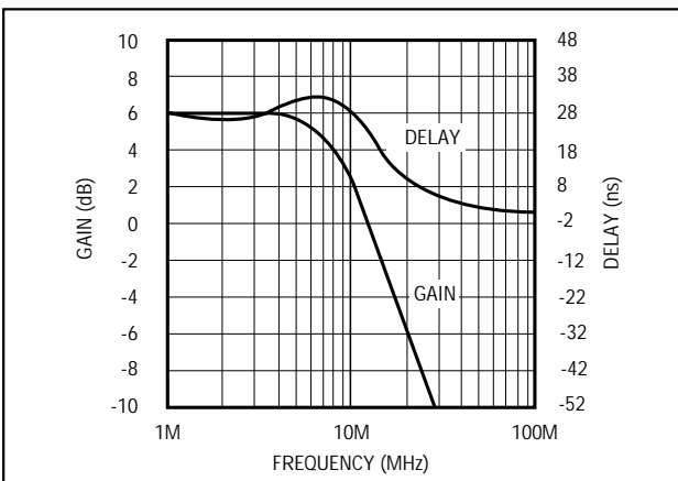
Figure 10b. Gain and Delay vs. Frequency
