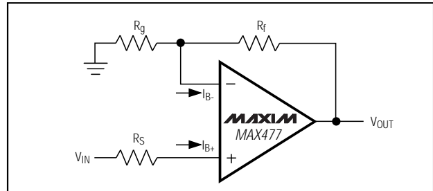
Figure 3. Output Offset Voltage
