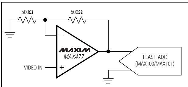
Figure 7. Preamp for Video Digitizer
