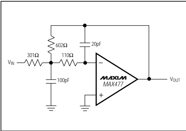
Figure 9. 8MHz Bessel Filter
