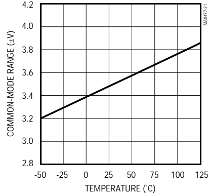
INPUT COMMON-MODE RANGE ( V_{CM} ) vs. TEMPERATURE
