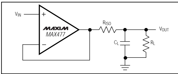
Figure 5. Capacitive-Load Driving Circuit
