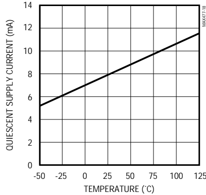
QUIESCENT SUPPLY CURRENT ( I_{Sv} ) vs. TEMPERATURE
