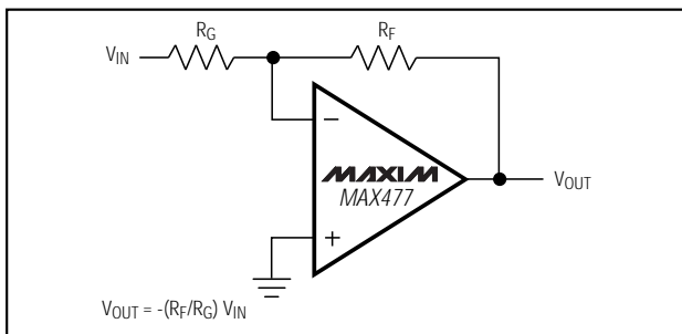
Figure 1a. Inverting Gain Configuration
