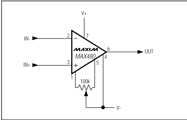
Figure 1. Offset Nulling Circuit
