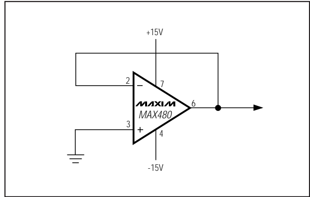
Figure 2. Burn-In Circuit
