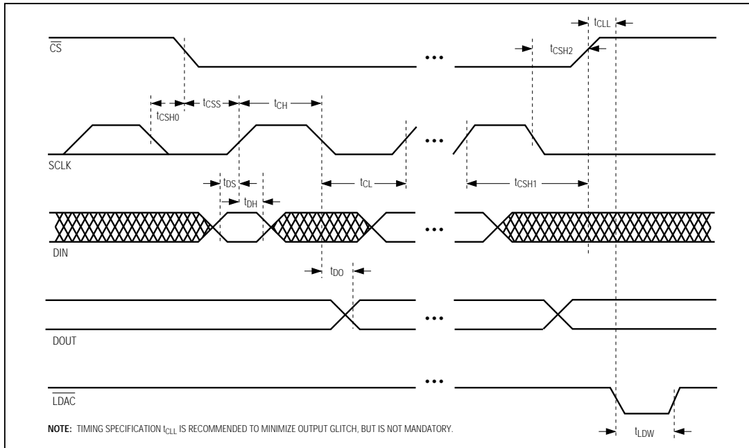
Figure 2. Detailed Serial Interface Timing (Mode 0 Shown)
