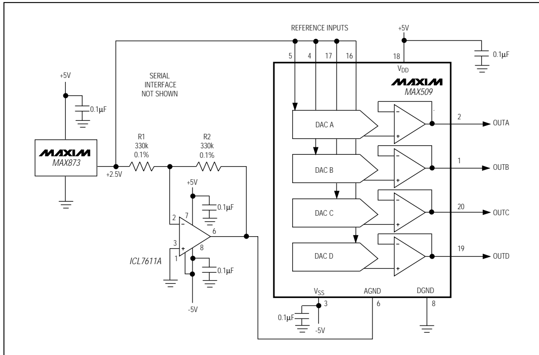
Figure 14. MAX509 AGND Bias Circuit (Negative Offset)
