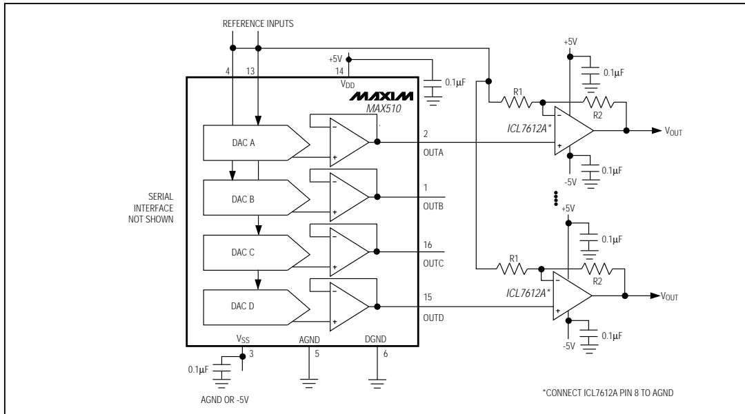
Figure 17. MAX510 Bipolar Output Circuit
