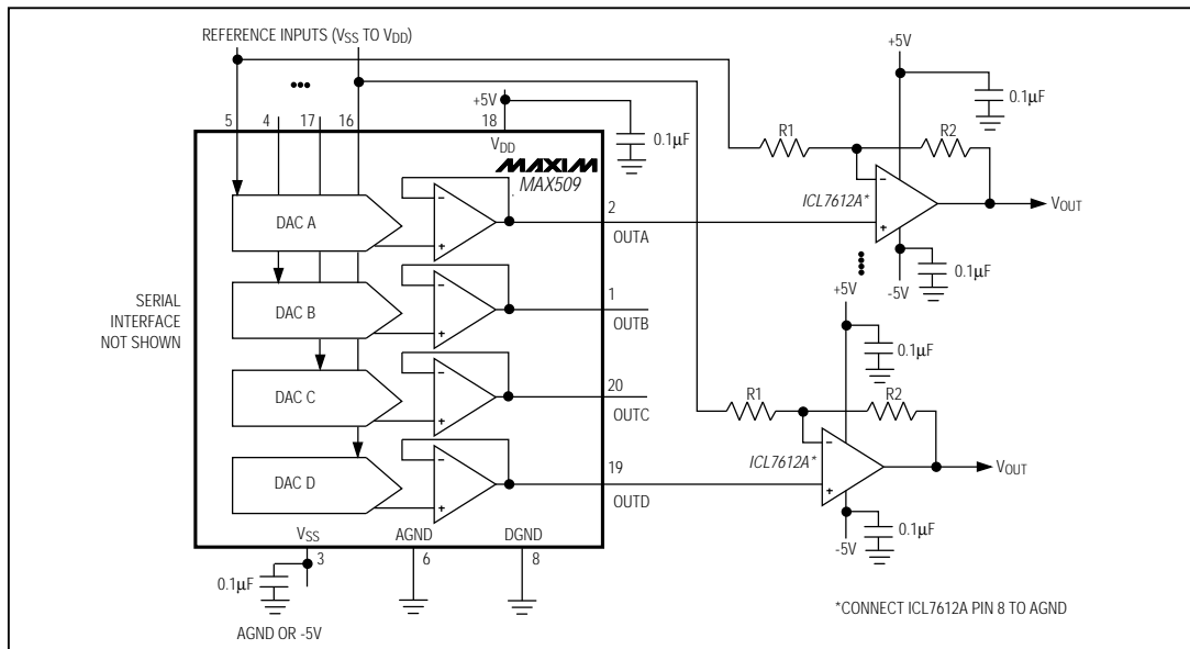
Figure 16. MAX509 Bipolar Output Circuit
