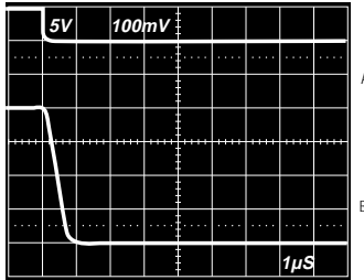
NEGATIVE SETTLING TIME (V SS = AGND)
