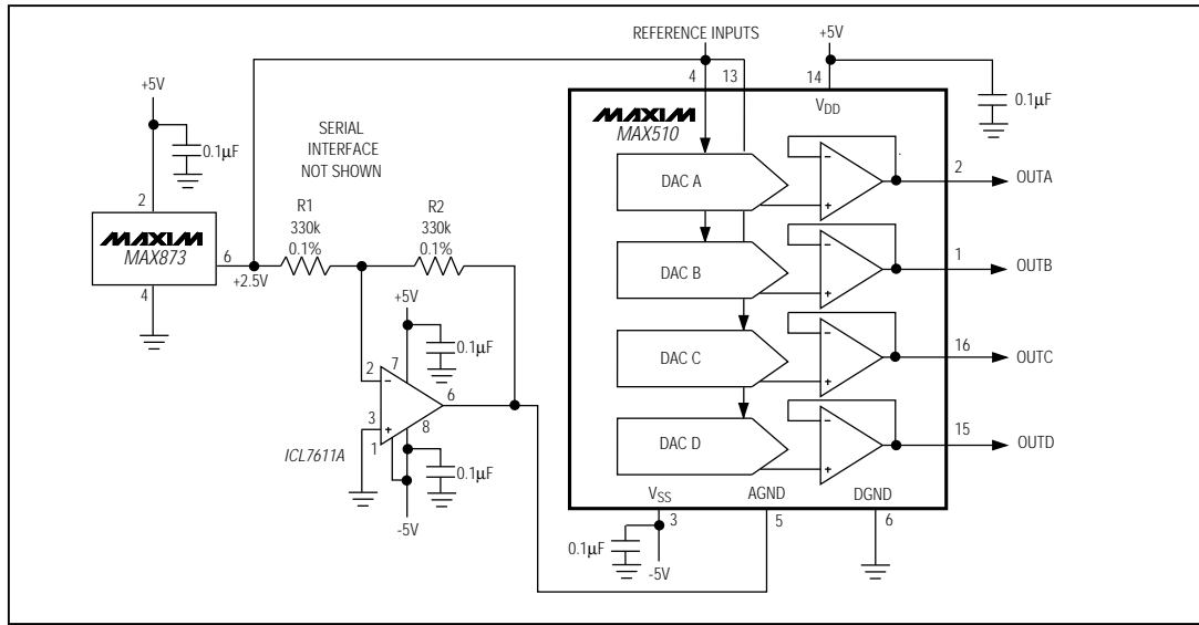
Figure 15. MAX510 AGND Bias Circuit (Negative Offset)
