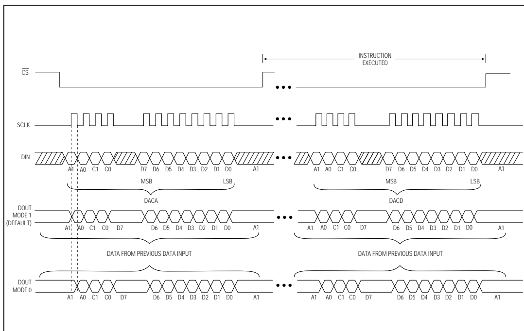
Figure 1. MAX509/MAX510 3-Wire Interface Timing
