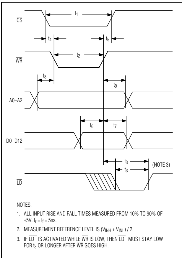
Figure 2. Digital Timing Diagram
