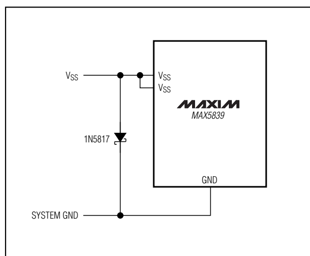
Figure 3. Schottky Diode Between V SS and GND
