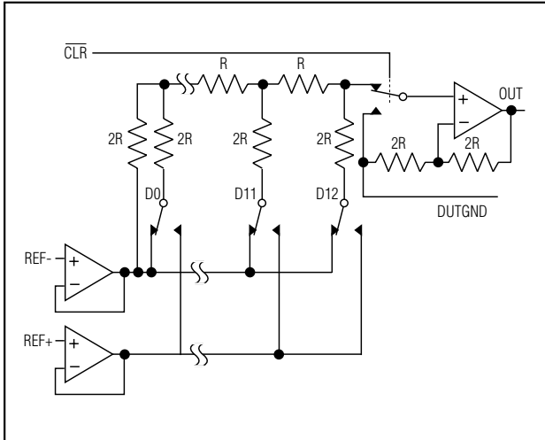
Figure 1. DAC Simplified Circuit
