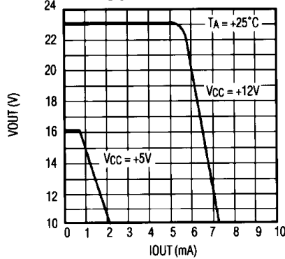
MAX623 OUTPUT VOLTAGE vs. OUTPUT CURRENT
