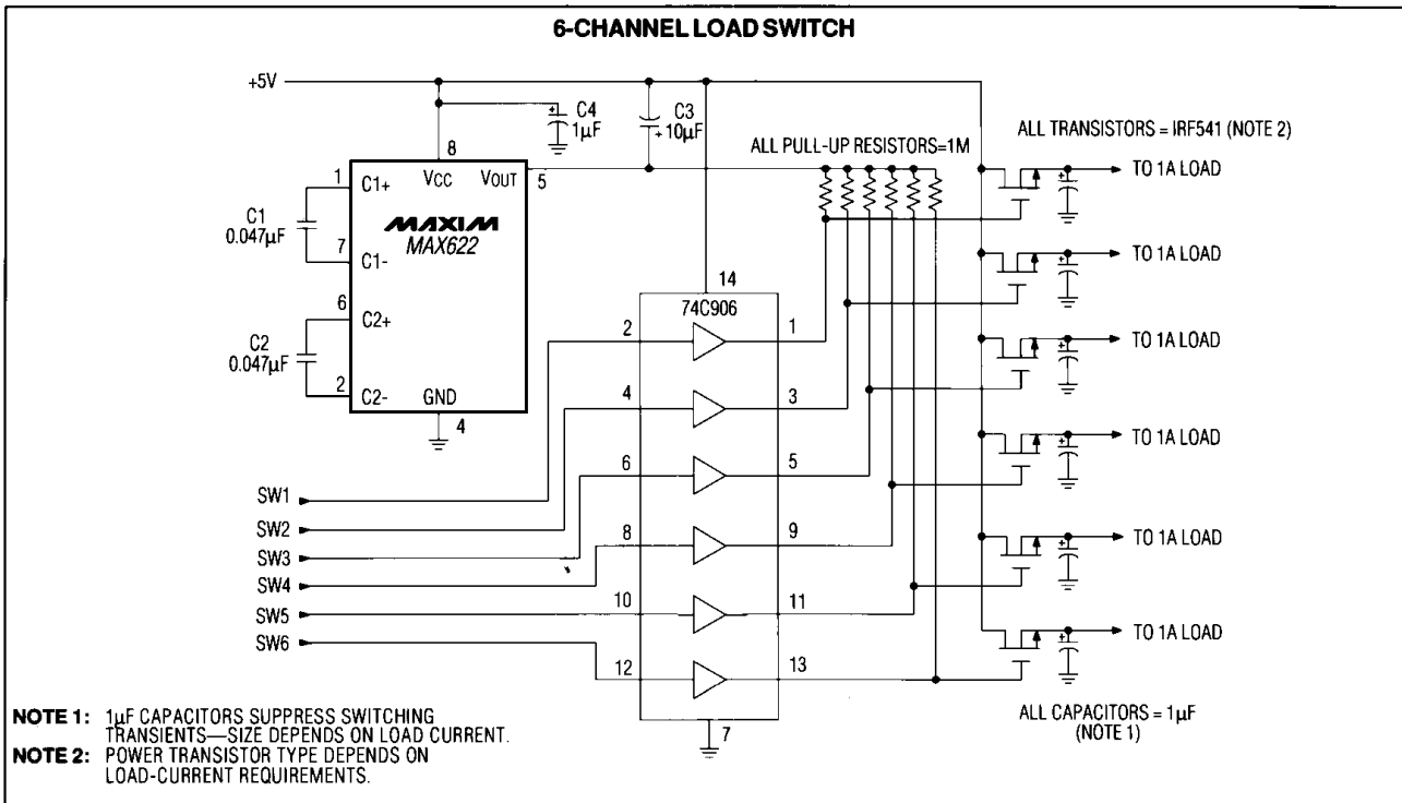
Figure 4. A Single MAX622 Drives Six High-Side Switches
