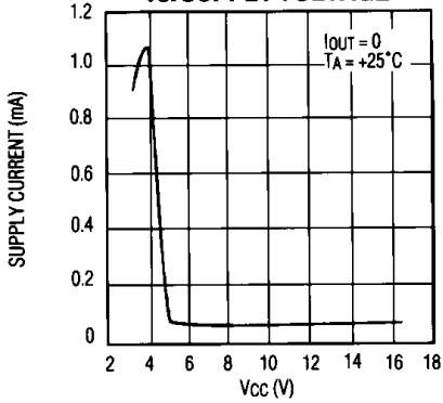
MAX623 SUPPLY CURRENT vs. SUPPLY VOLTAGE
