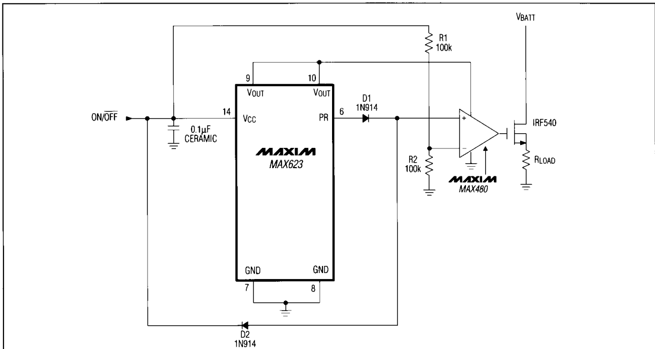
Figure 3. Single-Load Switch
