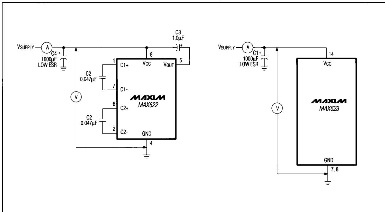
Figure 2. MAX622/MAX623 Quiescent Supply-Current Test Circuits
