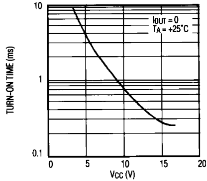
MAX622/MAX623 TURN-ON TIME vs. SUPPLY VOLTAGE
