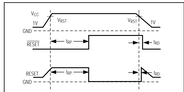
Figure 2. Reset Timing Diagram
