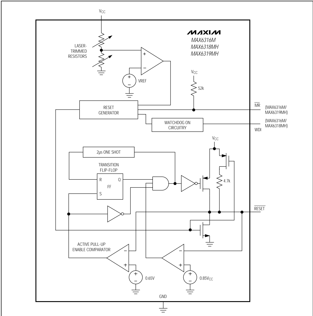
Figure 4. MAX6316/MAX6318MH/MAX6319MH Bidirectional Reset Output Functional Diagram
