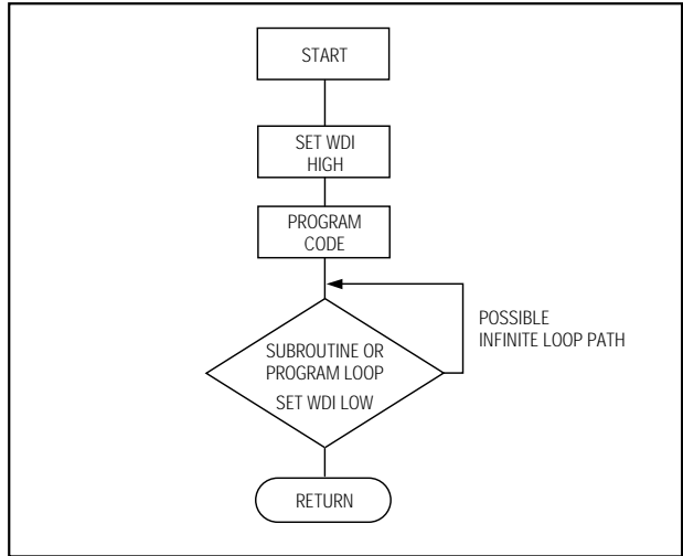
Figure 10. Watchdog Flow Diagram
