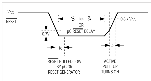
Figure 5. Bidirectional \overline{\text{RESET}} Timing Diagram
