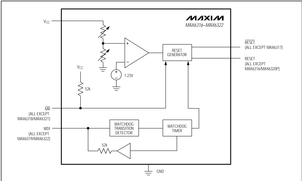
Figure 1. Functional Diagram
