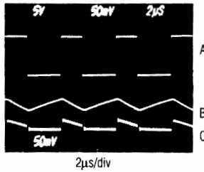
A: Switch Voltage (LX pin), 5V/div, 0V to +12.4V B: Inductor Current, 500mA/div C: Output Voltage Ripple, 50mV/div Circuit of Fig. 2b, C_{OUT} = 300\mu F , V_+ = 3V , I_{OUT} = 100mA , T_A = +25^\circ C
