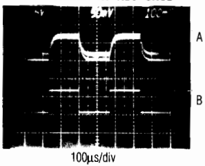
A: V_{OUT} , 50mV/div, DC-Coupled B: V_+ , 5V/div, 6.0V to 12.0V Circuit of Fig. 2b, I_{OUT} = 125mA , V_{OUT} = 15V , T_A = +25^\circ C
