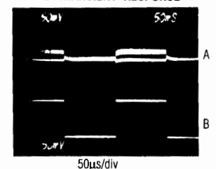
A: V_{OUT} , 50mV/div, DC-Coupled B: I_{OUT} , 100mA/div, 10mA to 200mA Circuit of Fig. 2b, V_+ = +6V , T_A = +25^\circ C , V_{OUT} = 12V
