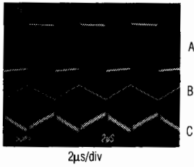
A: Switch Voltage (LX pin), 2V/div, 0V to +5V B: Inductor Current, 500mA/div C: Output Voltage Ripple, 50mV/div Circuit of Fig. 2a, C_{OUT} = 150\mu F , V_+ = 3V , I_{OUT} = 200mA , T_A = +25^\circ C
