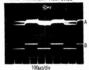
A: V_{OUT} , 50mV/div, DC-Coupled B: V_+ , 5V/div, 6.0V to 9.0V Circuit of Fig. 2b, I_{OUT} = 200mA , V_{OUT} = 12V , T_A = +25^\circ C
