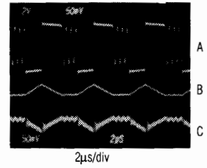
A: Switch Voltage (LX pin), 2V/div, 0V to +5V B: Inductor Current, 500mA/div C: Output Voltage Ripple, 50mV/div Circuit of Fig. 2a, C_{OUT} = 150\mu F , V_+ = 3V , I_{OUT} = 100mA , T_A = +25^\circ C
