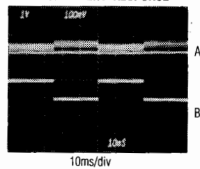
A: V_{OUT} , 100mV/div B: V_{IN} , 2V to 3V Circuit of Fig. 2a, I_{LOAD} = 200mA , T_A = +25^\circ C
