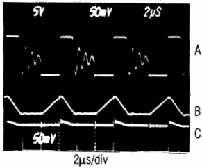
A: Switch Voltage (LX pin), 5V/div, 0V to +12.4V B: Inductor Current, 200mA/div C: Output Voltage Ripple, 50mV/div Circuit of Fig. 2b, C_{OUT} = 300\mu F , V_+ = 3V , I_{OUT} = 200mA , T_A = +25^\circ C
