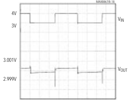
100 \mu s /div MAX886_EUK30, I_{LOAD} = 50mA
