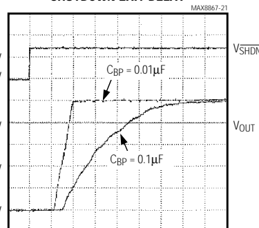
I_{LOAD} = 50mA 5 \mu s /div
