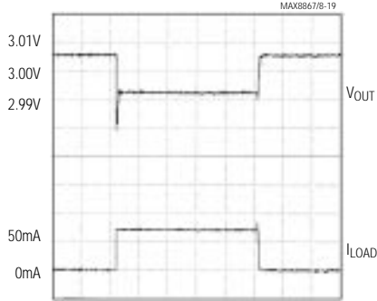
10 \mu s /div MAX886_EUK30, V_{IN} = V_{OUT} + 0.5V , C_{IN} = 10\mu F , I_{LOAD} = 0mA TO 50mA
