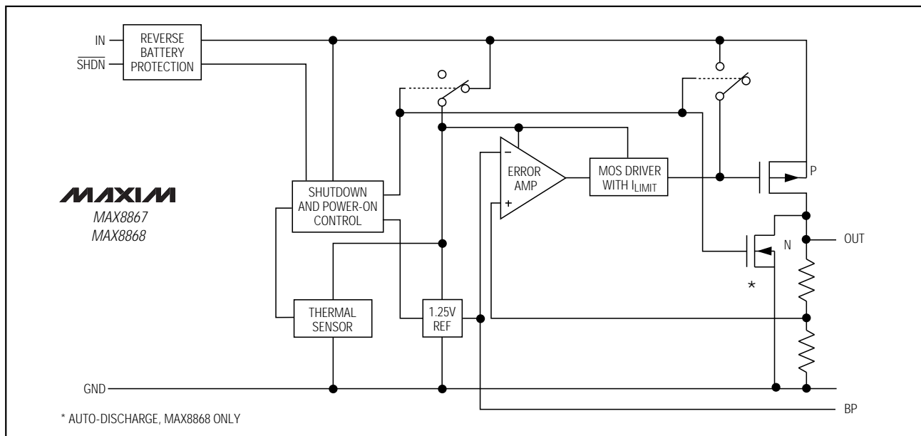
Figure 1. Functional Diagram
