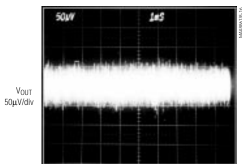
1ms/div C_{OUT} = 10\mu F , C_{BP} = 0.1\mu F , I_{LOAD} = 10mA
