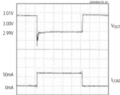
10 \mu s /div MAX886_EUK30, V_{IN} = V_{OUT} + 0.1V , C_{IN} = 10\mu F , I_{LOAD} = 0mA TO 50mA
