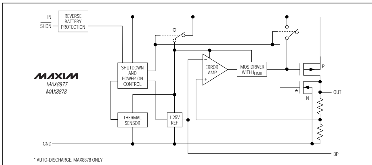
Figure 1. Functional Diagram
