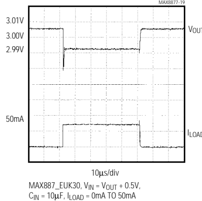
LOAD-TRANSIENT RESPONSE
