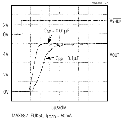
MAX887_EUK50 SHUTDOWN EXIT DELAY
