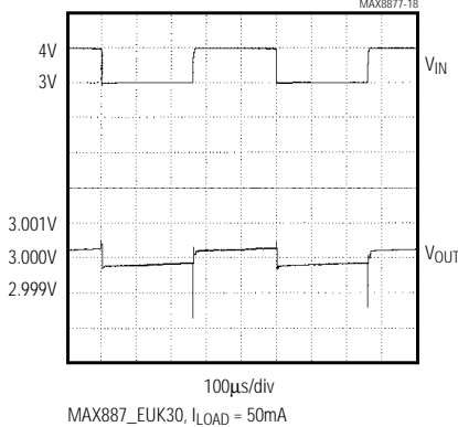
LINE-TRANSIENT RESPONSE
