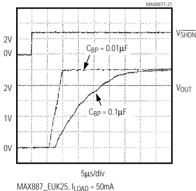
MAX887_EUK25 SHUTDOWN EXIT DELAY
