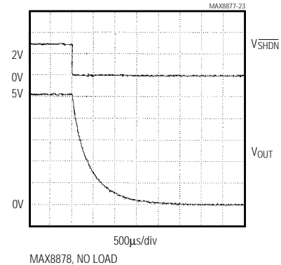
ENTERING SHUTDOWN
