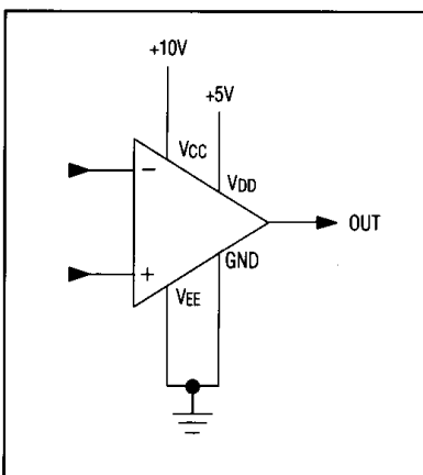
Figure 1A. Separate Analog Supply, Common Ground
