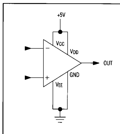
Figure 1B. Single +5V Supply, Common Ground
