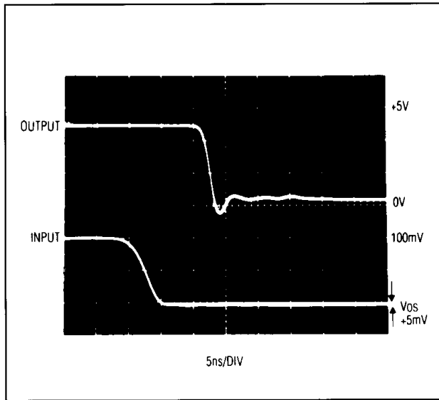
Figure 4. t_{pd+} Response Time to 5mV Overdrive
