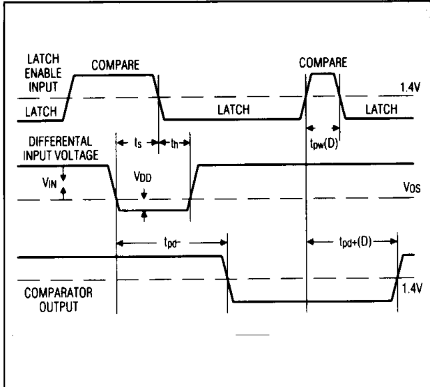
Figure 2. MAX900/902/903 Timing Diagram
