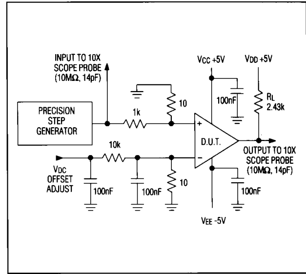
Figure 5. Response-Time Setup
