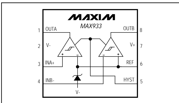
Figure 1b. MAX933 Functional Diagram
