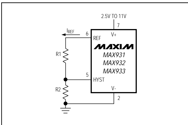
Figure 3. Programming the HYST Pin
