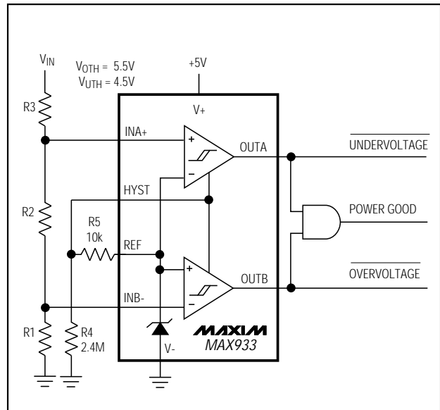
Figure 6. Window Detector
