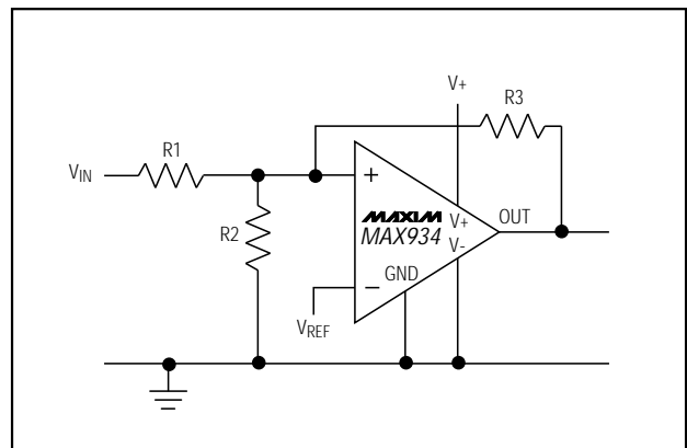
Figure 4. External Hysteresis
