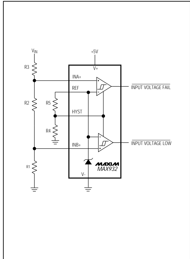
Figure 9. Two-Stage Low-Voltage Detector
