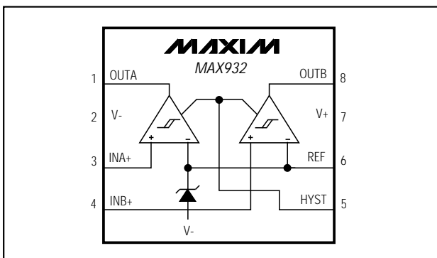
Figure 1a. MAX932 Functional Diagram
