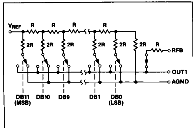
Figure 1. Simplified D/A Circuit of MX7545A/MAX7645
