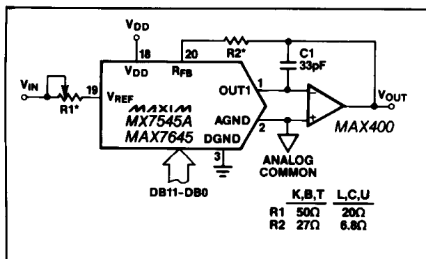
Figure 3. Unipolar Binary Operation
