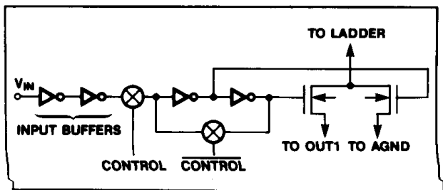
Figure 2. Digital Input Structure
