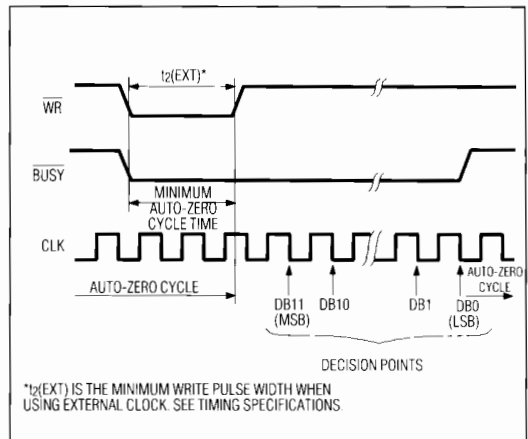
Figure 9. Operating Waveform - External Clock
