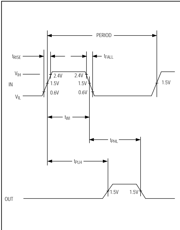
Figure 1. Timing Diagram
