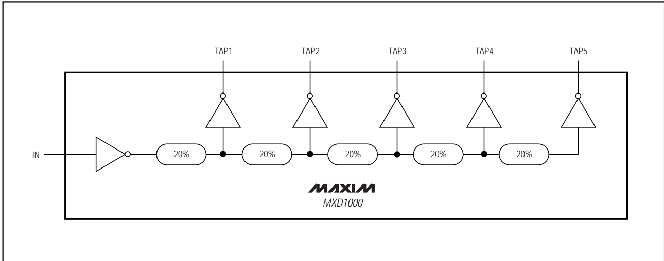
Functional Diagram
