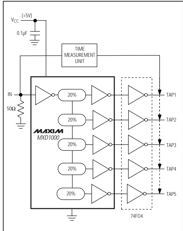
Figure 2. Test Circuit
