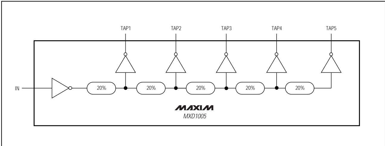
Functional Diagram
