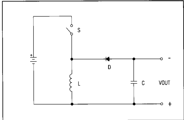
Figure 1. Simplified Inverting Converter
