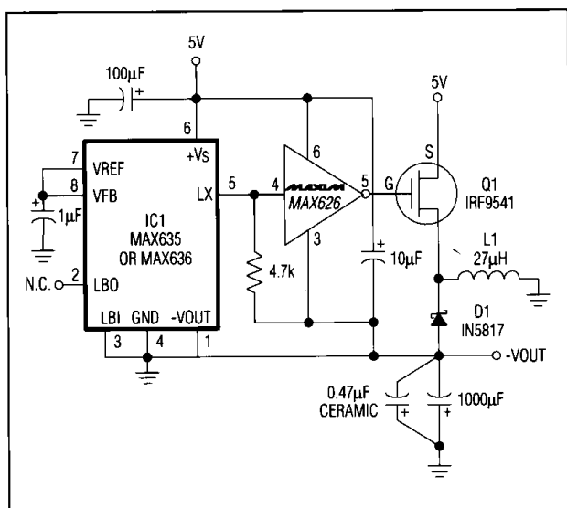
Figure 4. Medium Power Inverter
