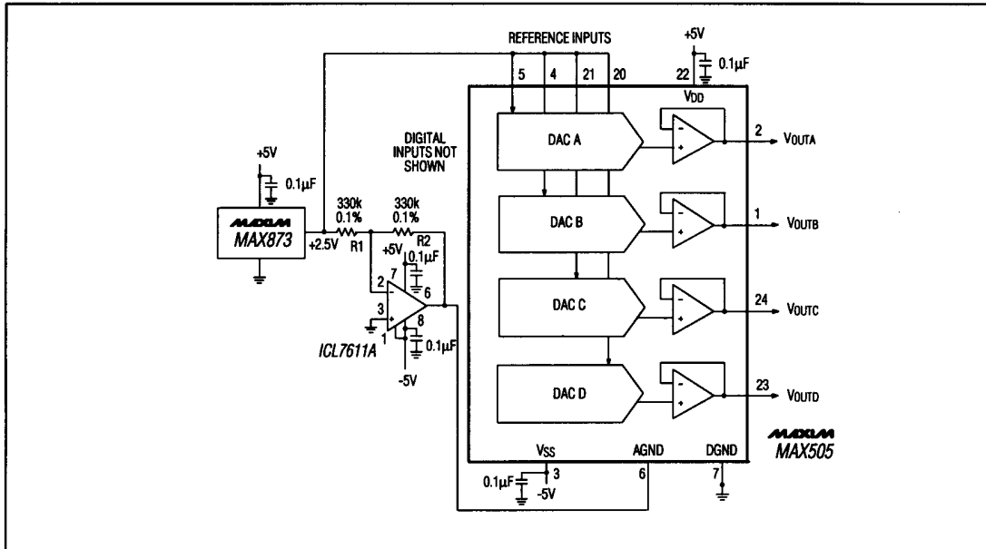
Figure 9a. MAX505 AGND Bias Circuit (Negative Offset)
