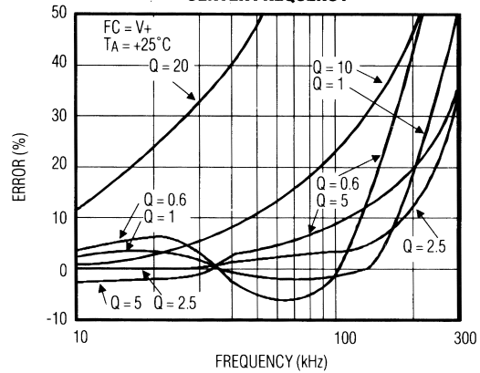
Q ERROR vs. PROGRAMMED CENTER FREQUENCY
