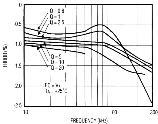
CENTER-FREQUENCY ERROR vs. PROGRAMMED CENTER FREQUENCY
