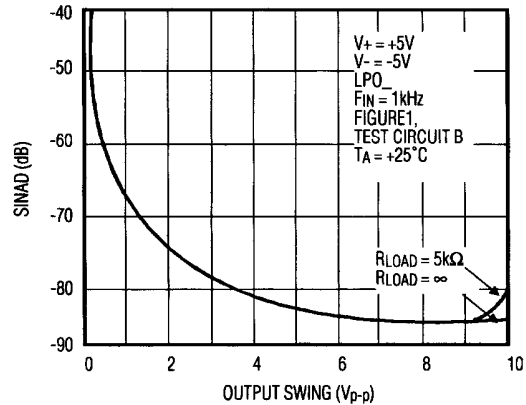
SIGNAL-TO-NOISE + DISTORTION (SINAD) vs. OUTPUT SWING
