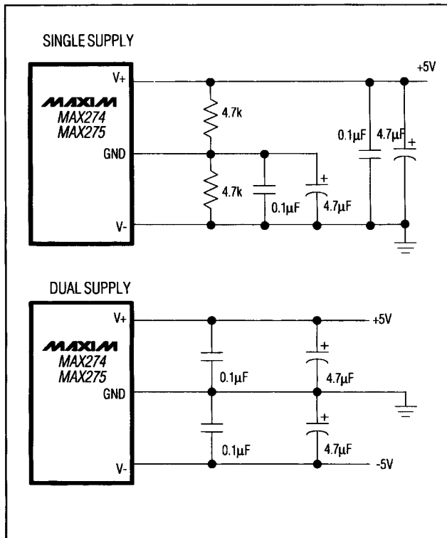
Figure 9. Power-Supply Configurations
