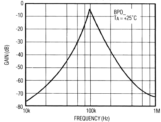
FILTER RESPONSE
