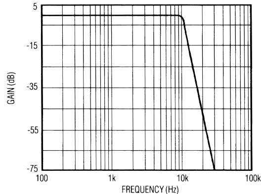
FILTER RESPONSE USING TYPICAL OPERATING CIRCUIT
