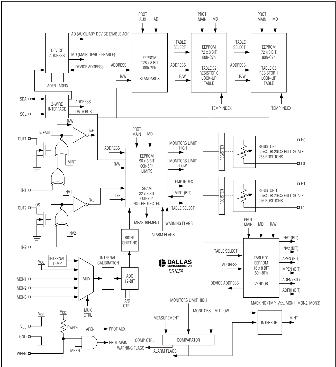
Figure 1. Block Diagram
