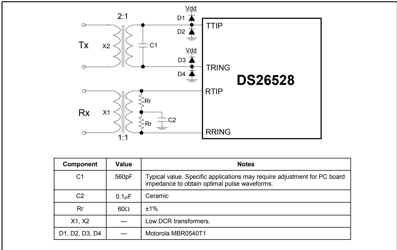
Figure 9-11. Basic Balanced Network Connections
