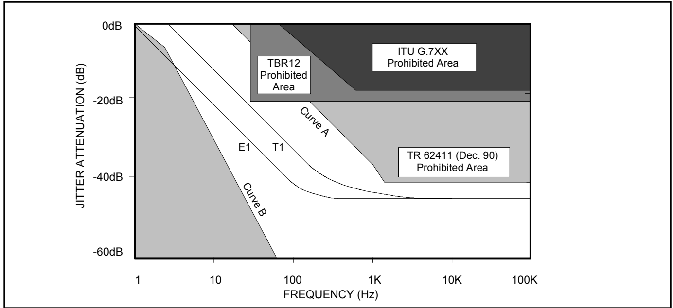
Figure 9-16. Jitter Attenuation
