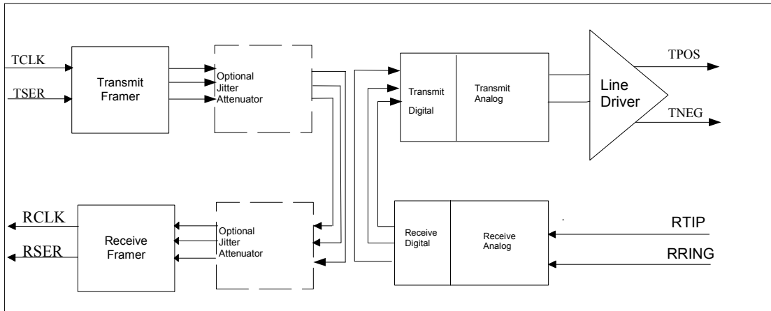
Figure 9-20. Dual Loopback
