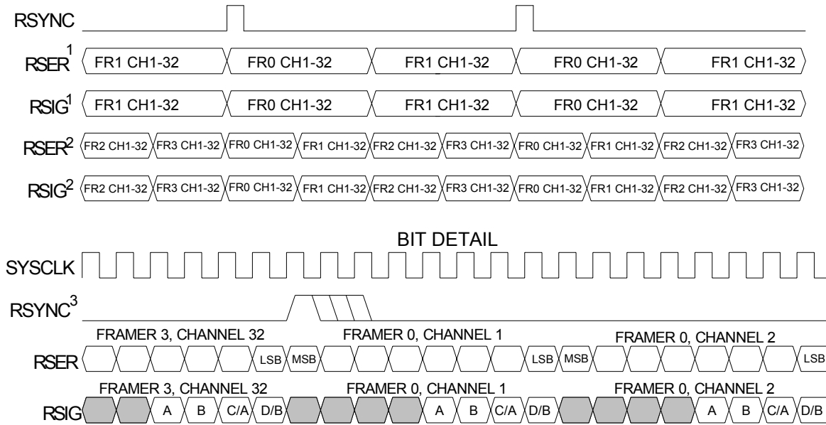
Figure 11-7. T1 Receive Side Interleave Bus Operation, FRAME Mode
