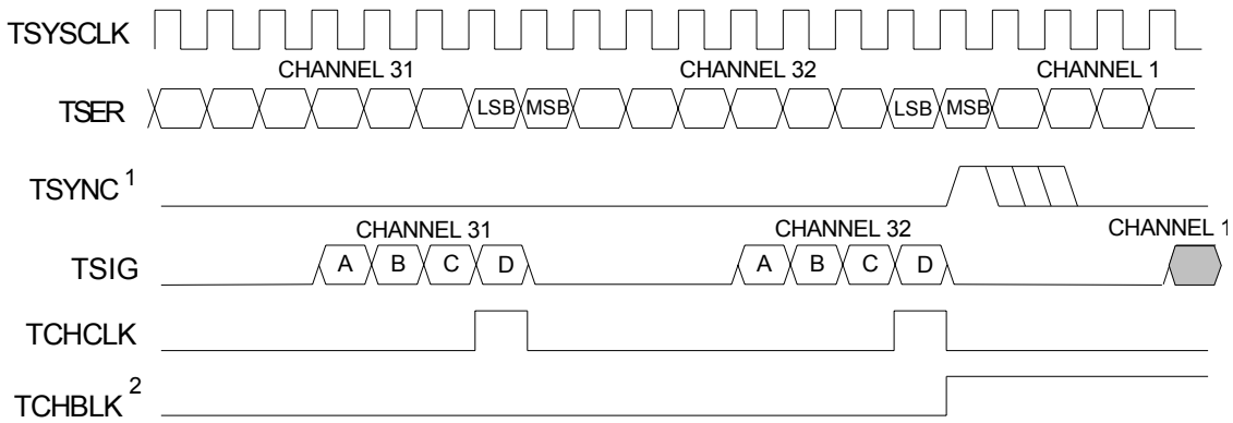
Figure 11-22. E1 Transmit Side 2.048MHz Boundary Timing (e-store enabled)
