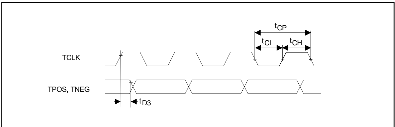
Figure 13-10. Transmit Formatter Timing—Line Side
