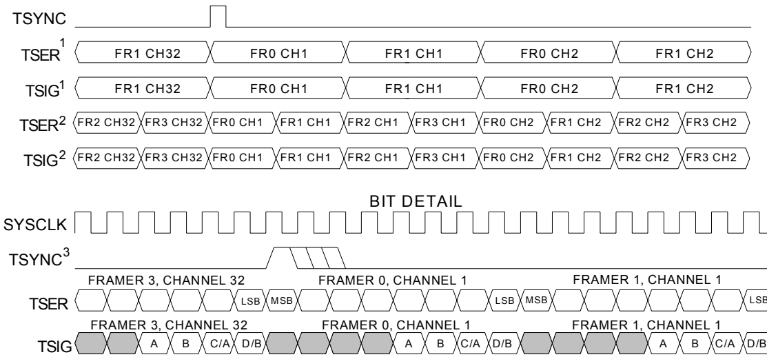
Figure 11-13. T1 Transmit Side Interleave Bus Operation, BYTE Mode
