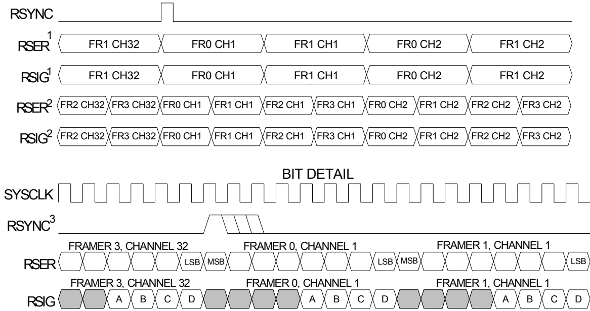
Figure 11-6. T1 Receive Side Interleave Bus Operation, BYTE Mode
