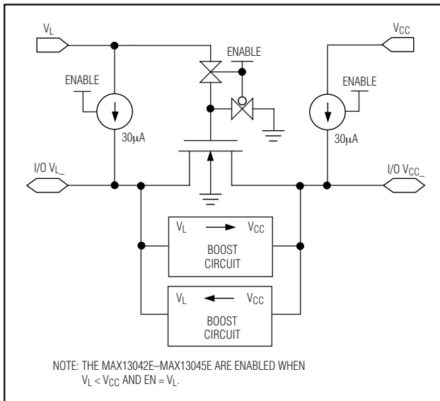
Figure 4. Simplified Functional Diagram for One I/O Line
