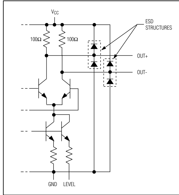
Figure 7. CML Output Circuit
