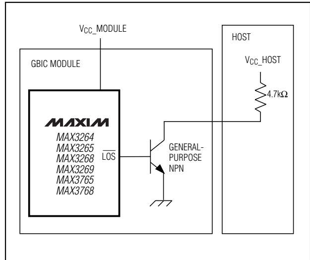
Figure 8. Recommended GBIC LOS Circuit
