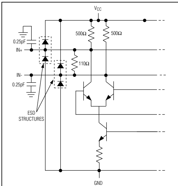
Figure 4. Input Circuit
