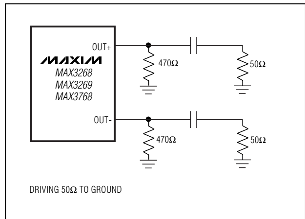
Figure 9. Alternative PECL Termination
