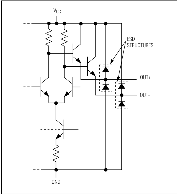
Figure 6. PECL Output Circuit
