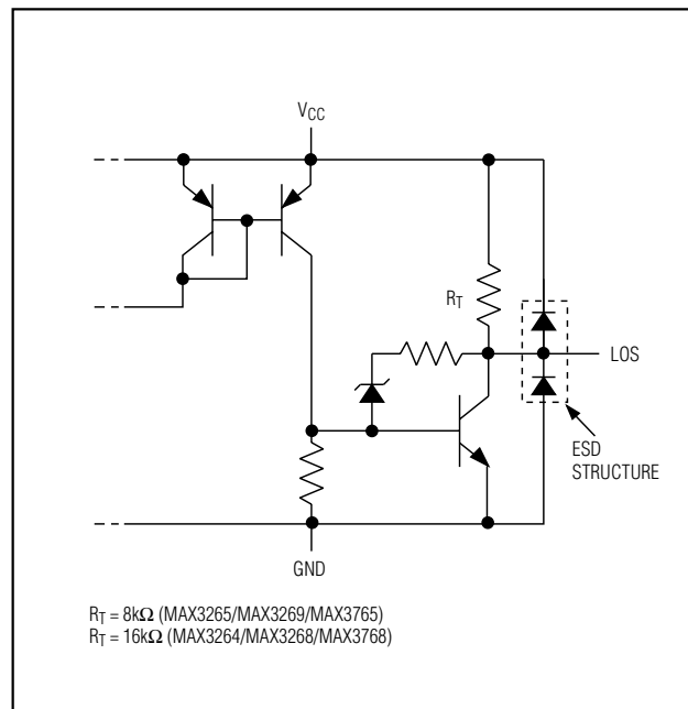
Figure 5. LOS Output Circuit
