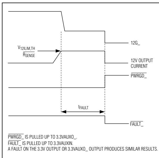
Figure 4. 12 Output Overcurrent/Short Circuit During Normal Operation
