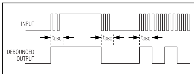
Figure 5. INPUT_ and OUTPUT_ Debounced Feature
