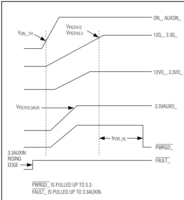
Figure 2. Power-Up Timing, No Fault
