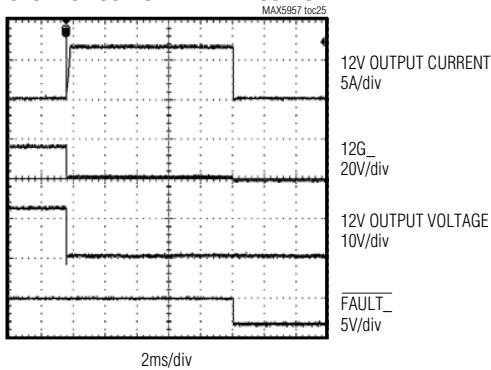
SHORT CIRCUIT ON 12V MAIN OUTPUT
