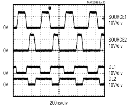
OUT-OF-PHASE OPERATION (FSEL_1 = VL)
