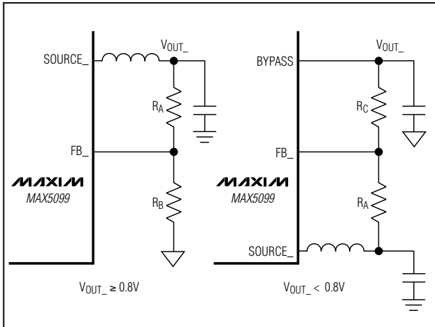
Figure 2. Adjustable Output Voltage
