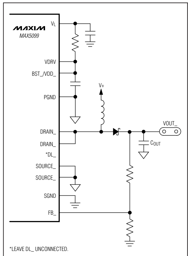
Figure 5. Boost Application
