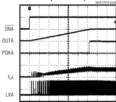
REG A STARTUP WAVEFORM (HEAVY LOAD)
