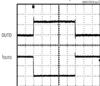
REG D LOAD TRANSIENT (SOURCE/SINK)
