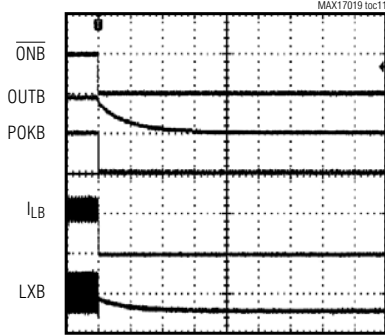
REG B SHUTDOWN WAVEFORM
