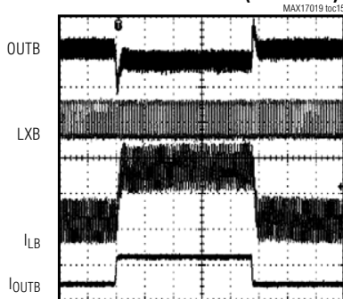
REG B LOAD TRANSIENT (0.4A TO 2A)
