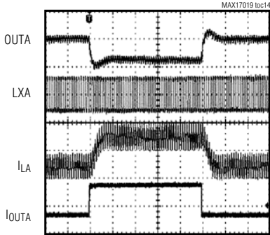
REG A LOAD TRANSIENT (1A TO 3.2A)
