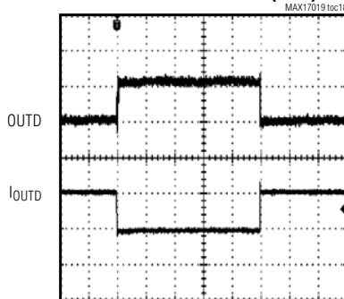
REG D LOAD TRANSIENT (SINK)
