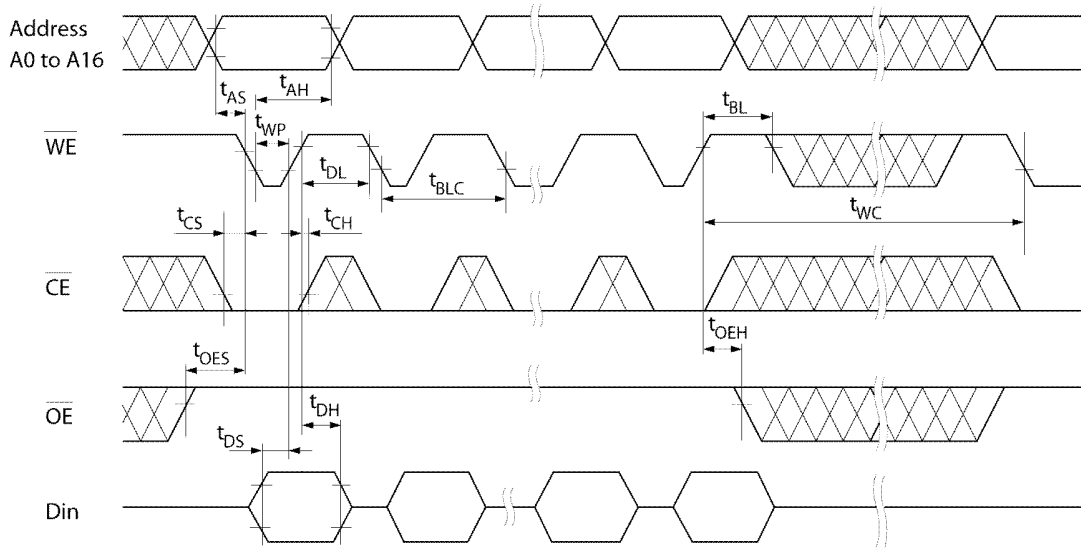
FIGURE 4. PAGE WRITE TIMING WAVEFORM (1) ( \overline{WE} CONTROLLED)
