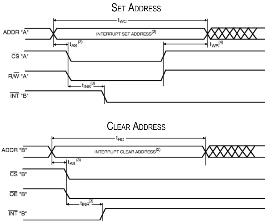
FIGURE 11. WAVEFORM OF INTERRUPT TIMING 1
