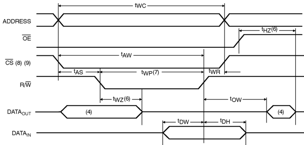
FIGURE 6. TIMING WAVEFORM OF WRITE CYCLE NO. 1, \text{R}/\overline{\text{W}} CONTROLLED TIMING 1,2,3,7
