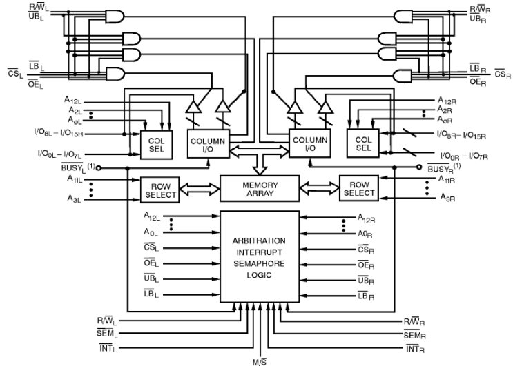
Logic Diagram
