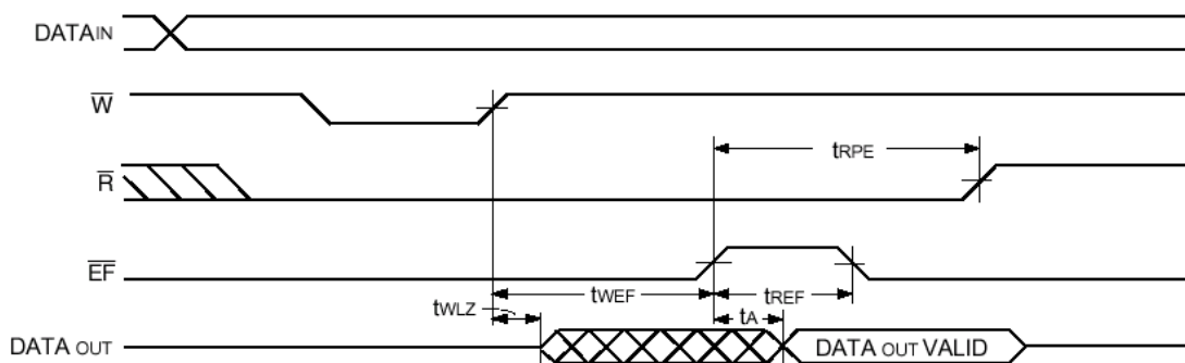
FIGURE 11. READ DATA FLOW FOR THROUGH MODE
