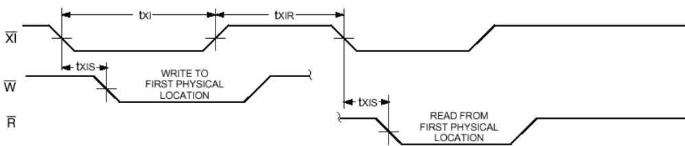
FIGURE 11. READ DATA FLOW FOR THROUGH MODE
